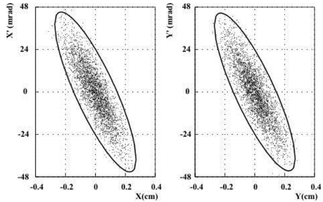
Figure 4: The transverse beam phase portraits at the RFQ entrance; ellipses represent 99% of the particles.
