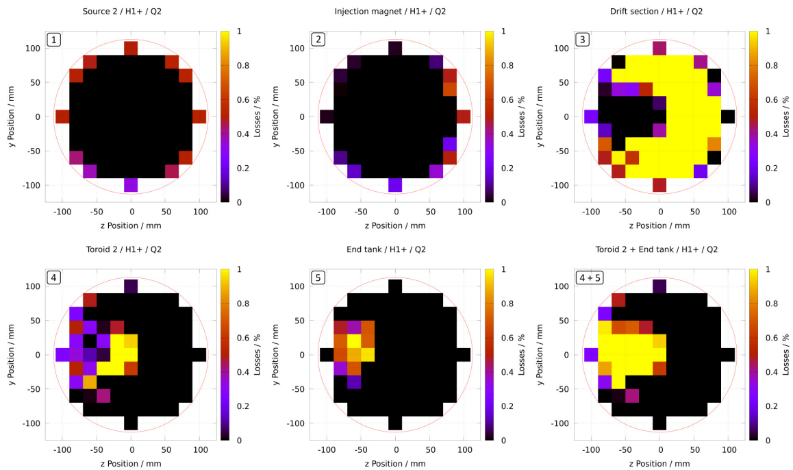
Figure 3: The picture shows the losses in each component of the transport and injection channel for 81 simulations with different starting positions in front of the injection magnet (z/y-coordinates). The magnetic field of the injection coil was B_{axis} = 0.326 T and the offset of the injection channel 100 mm.
