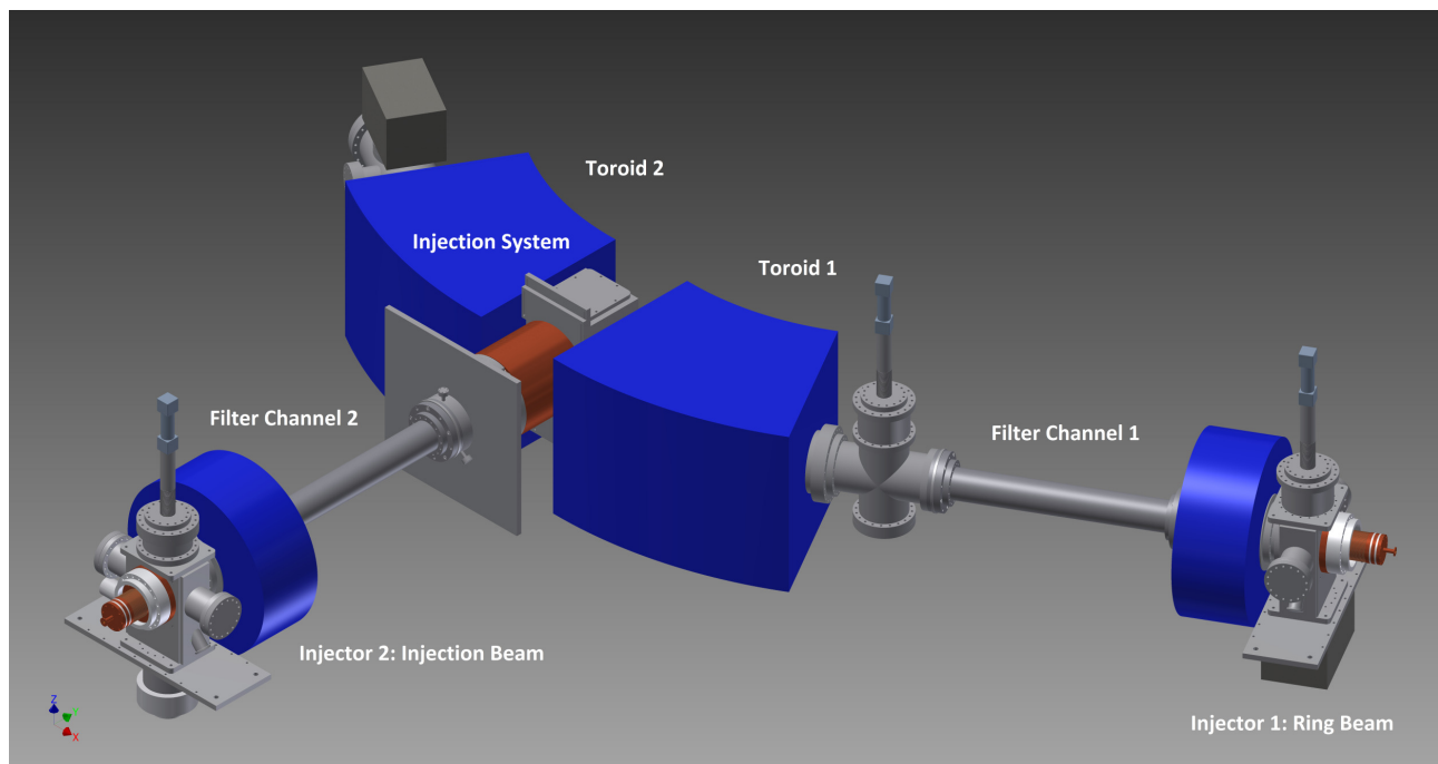
Figure 5: The complete layout of the experiment.
