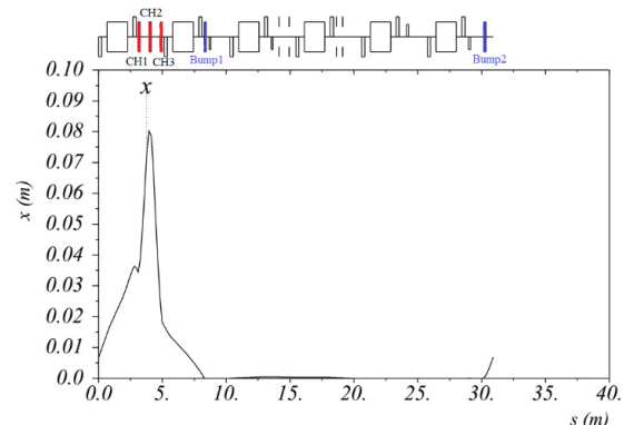
Figure 2: The closed orbit bump.
