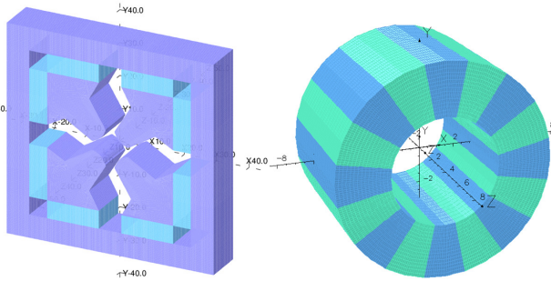
Figure 4: (Left) Isometric view of iron dominated magnet. (Right) Halbach type quadrupole.
