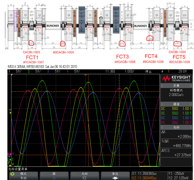
Figure 3: Layout of the MEBT, 5 FCT are labeled by red circle (up) and the beam phase measured by an oscilloscope (down).
