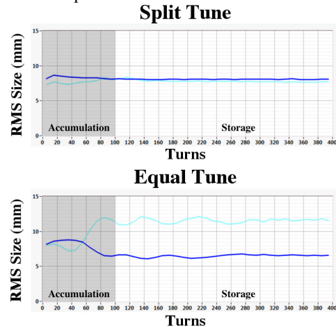
Figure 4: RMS size evolutions for the split tune (top) and equal tune (bottom) configurations for the simplified accumulation experiment. The horizontal RMS size is shown in dark blue and the vertical is shown in light blue.
