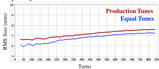
Figure 7: RMS beam sizes for the production tune (red) and equal tune (blue) configurations for the production style experiment.
