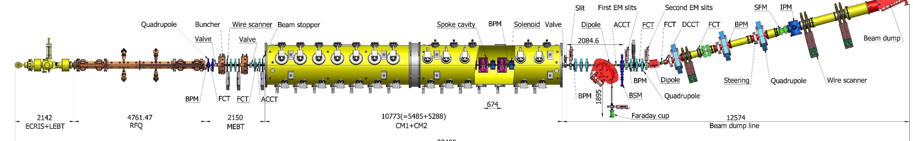
Figure 3: Layout of the ADS Injector-I testing facility
